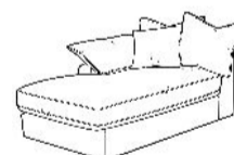
1 ARM CHAISE LHF PILLOW BACK (ALSO AVAILABLE IN RHF) H W D AH SH SD SW FH 88 110 172 55 46 124-128 90 68
